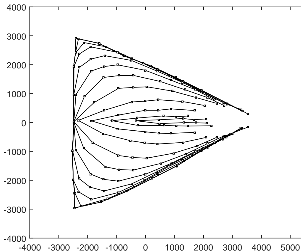
Figure 88: Polyester Rope, Heavy, Fast CombinedSeine dt 3 sec
