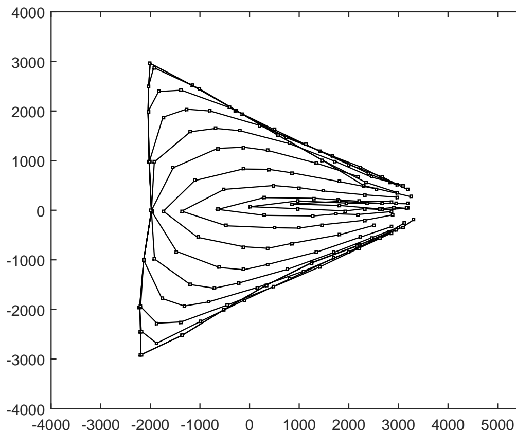
Figure 70: Combination Rope, Heavy, Slow, CombinedSeine, dt 4 sec
