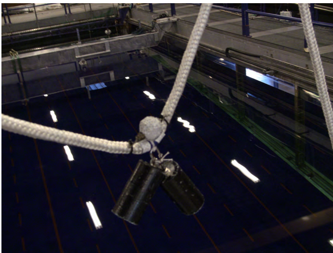
Figure 17: The clumps used for the high resistance case.
