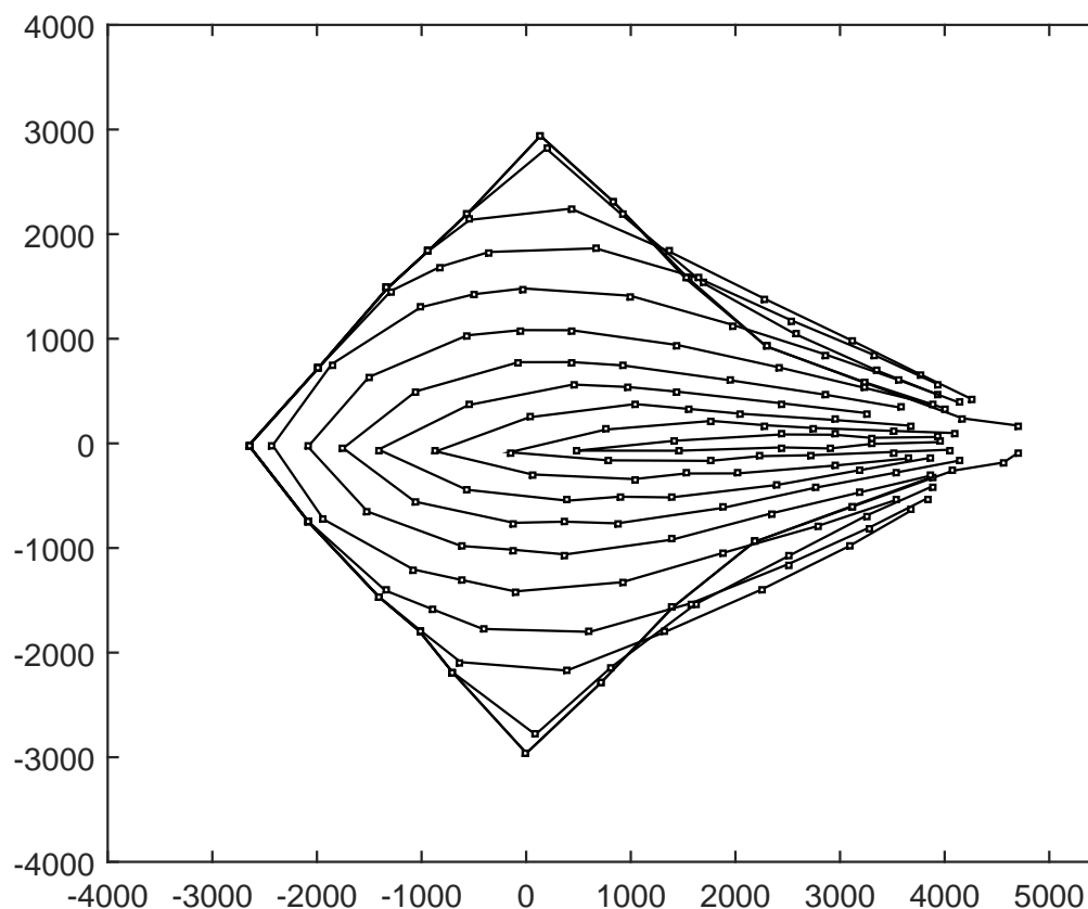
Figure 52: Combination Rope, Heavy, Fast CombinedSeine dt 2 sec
