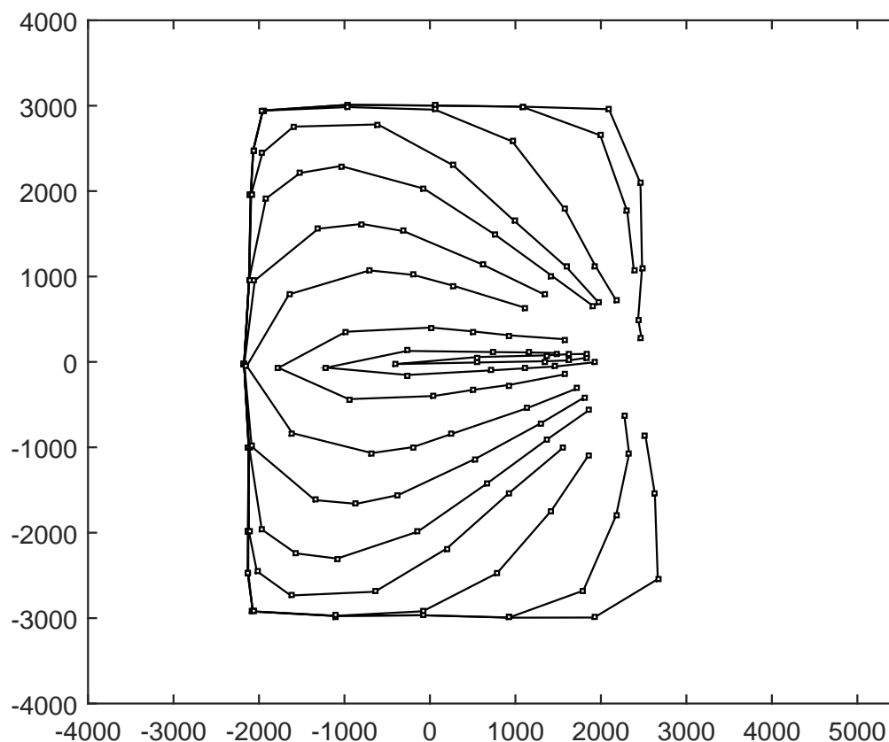
Figure 28: Combination Rope, Heavy, Fast CombinedSeine dt 3 sec
