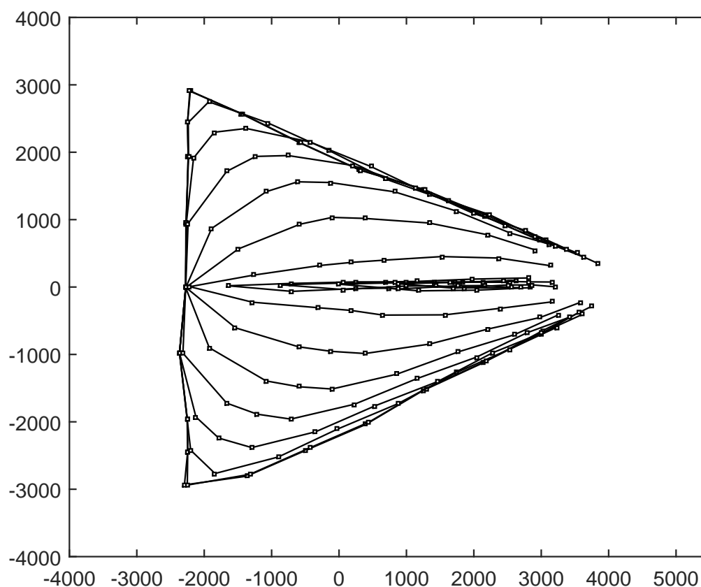
Figure 82: Polyester Rope, Heavy, Slow CombinedSeine dt 4 sec
