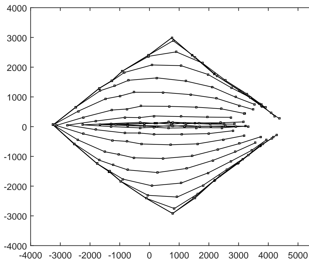
Figure 58: Polyester Rope, Heavy, Slow CombinedSeine dt 3 sec
