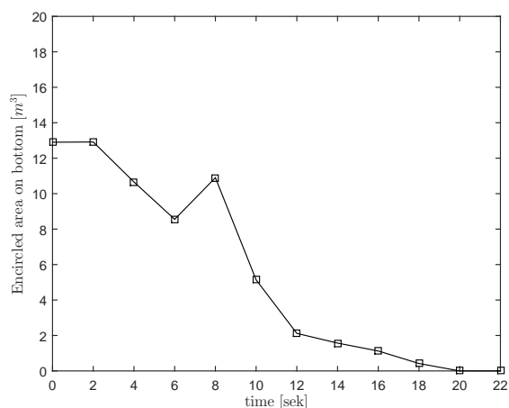
Figure 62: Polyester Rope, Light, Fast BottomArea
