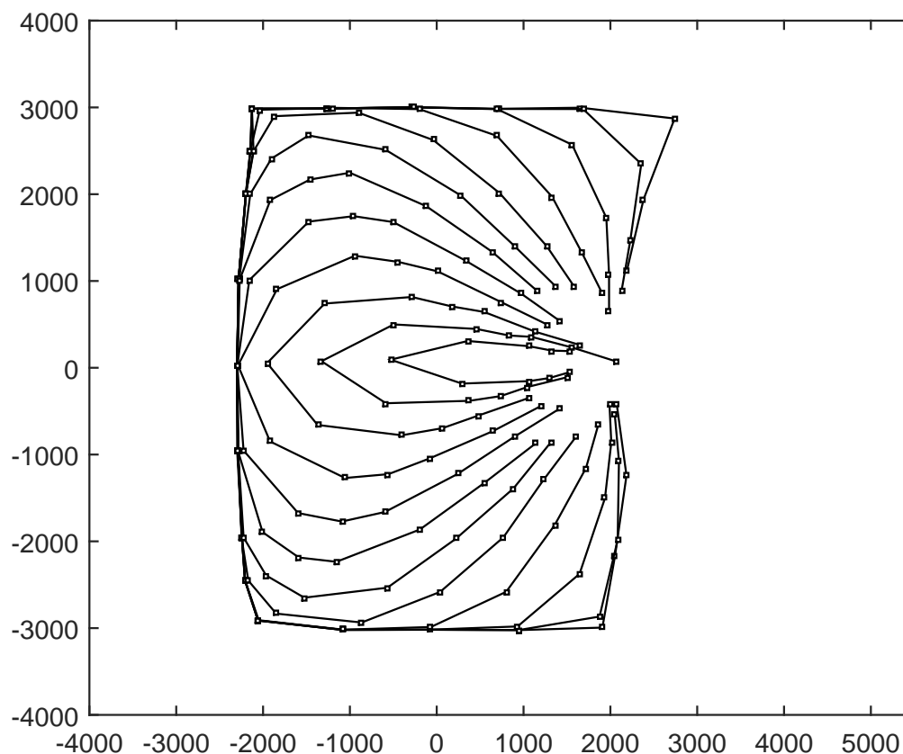
Figure 31: Polyester Rope, Light, Slow CombinedSeine dt 4 sec
