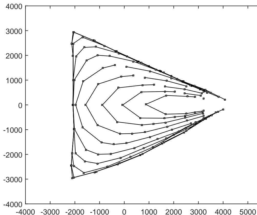
Figure 85: Polyester Rope, Light, Fast CombinedSeine dt 2.5 sec
