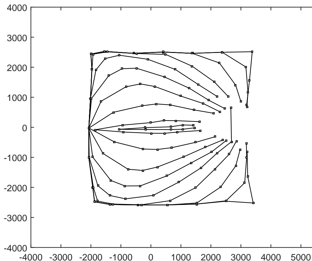
Figure 34: Polyester Rope, Heavy, Slow CombinedSeine dt 4.5 sec
